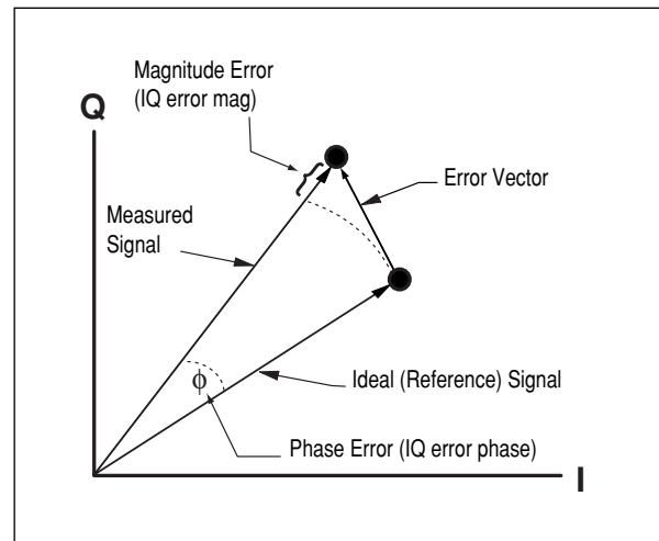
Figure 38. EVM and Related Qualities
