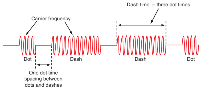
Figure 3-13 Sending the letter P by Morse code. An example of ON/OFF keying (OOK).
