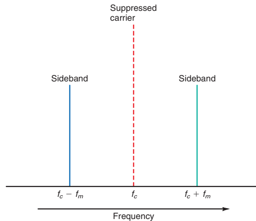
Figure 3-16 A frequency-domain display of DSB signal.
