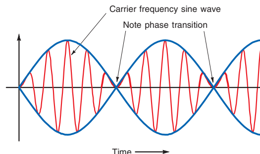
Figure 3-15 A time-domain display of a DSB AM signal.
