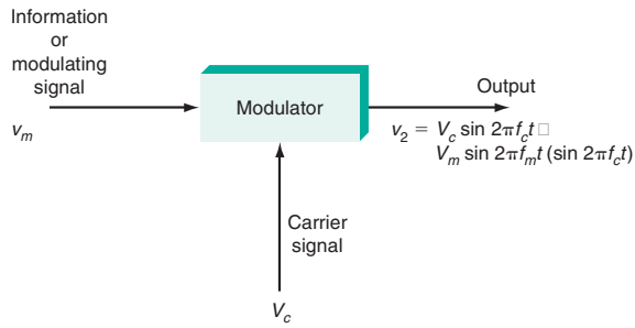
Figure 3-3 Amplitude modulator showing input and output signals.
